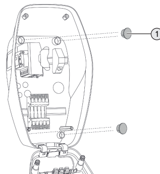
Fig. 9: Sealing plugs
