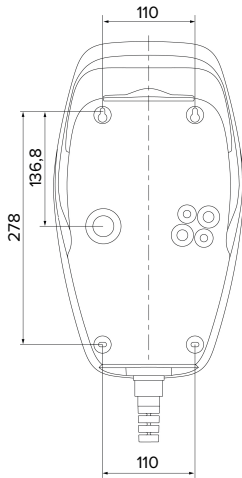
Abb. 7: Bohrmaße [mm]
