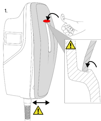
Fig. 22: Attach front cover - 1
