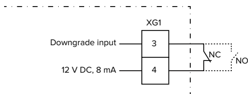
Fig. 18: Schematic circuit diagram: Connection of an external switching contact (default setting: NO)
