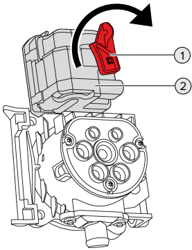
Fig. 26: Unlock the charging plug manually
