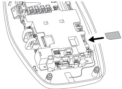
Fig. 13: Inserting the SIM card
