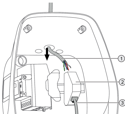
Fig. 16: Connecting the data line (example)
