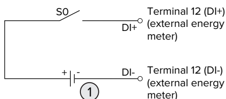
Fig. 19: Control via a coupling relay and additional power supply (when in delivery state)
