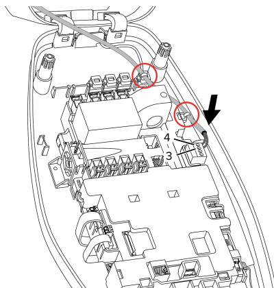
Fig. 17: Downgrade input connection
