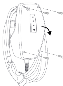
Fig. 6: Opening the product
