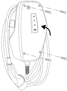
Fig. 20: Closing the product
