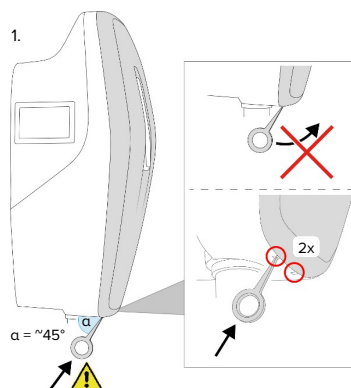
Abb. 4: Front Cover lösen - 1
