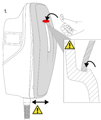
Fig. 22: Anbringe front cover - 1
