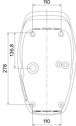
Abb. 8: Bohrmaße [mm]
